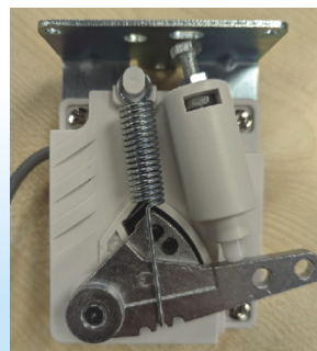
Treadle control lever.
