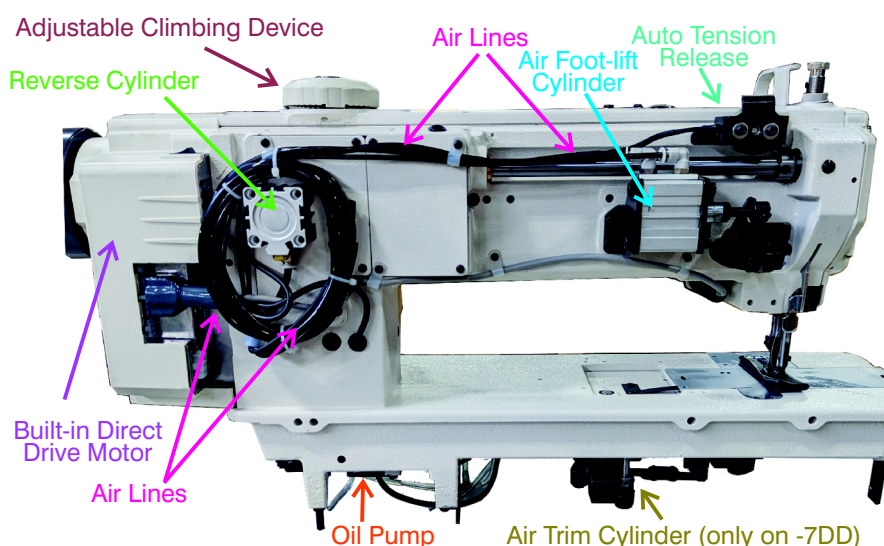
TWO NEEDLE WALKING FEET
