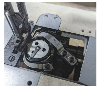
Thread Trimmer Knife
